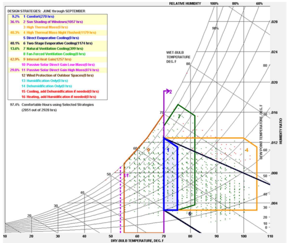
PSYCHROMETRIC CHART - SOLAR PASSIVE STRATEGIES FOR WARM MONTHS OF THE YEAR
